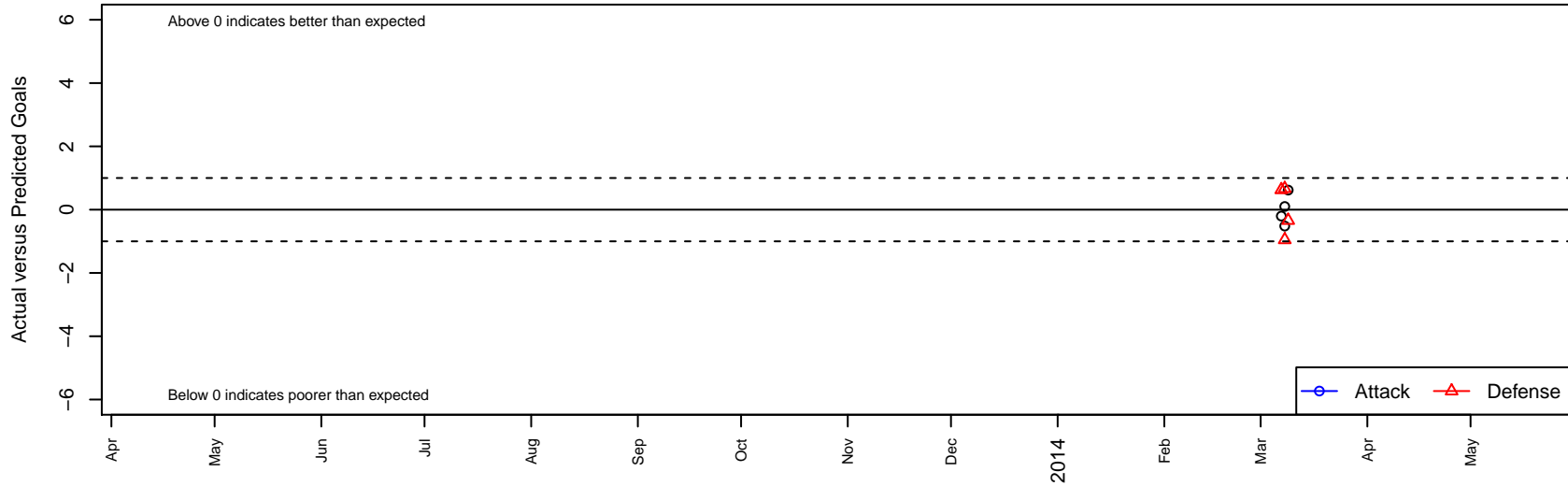
Futbolito Esforza B98 Dots are actual minus expected GF (blue circles) and GA (red triangles). Blue line is smoothed change in attack strength. Red is smoothed change in defense strength.
